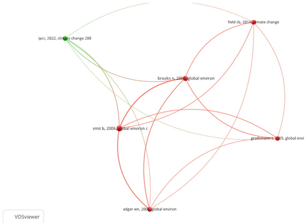
Figure 4. Co-citation
